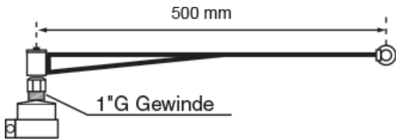
Extension arm with reduction for pole, including windsock
