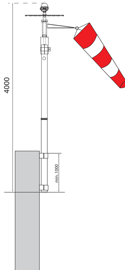
Pole for wall mounting, including windsock illumination and obstruction light
